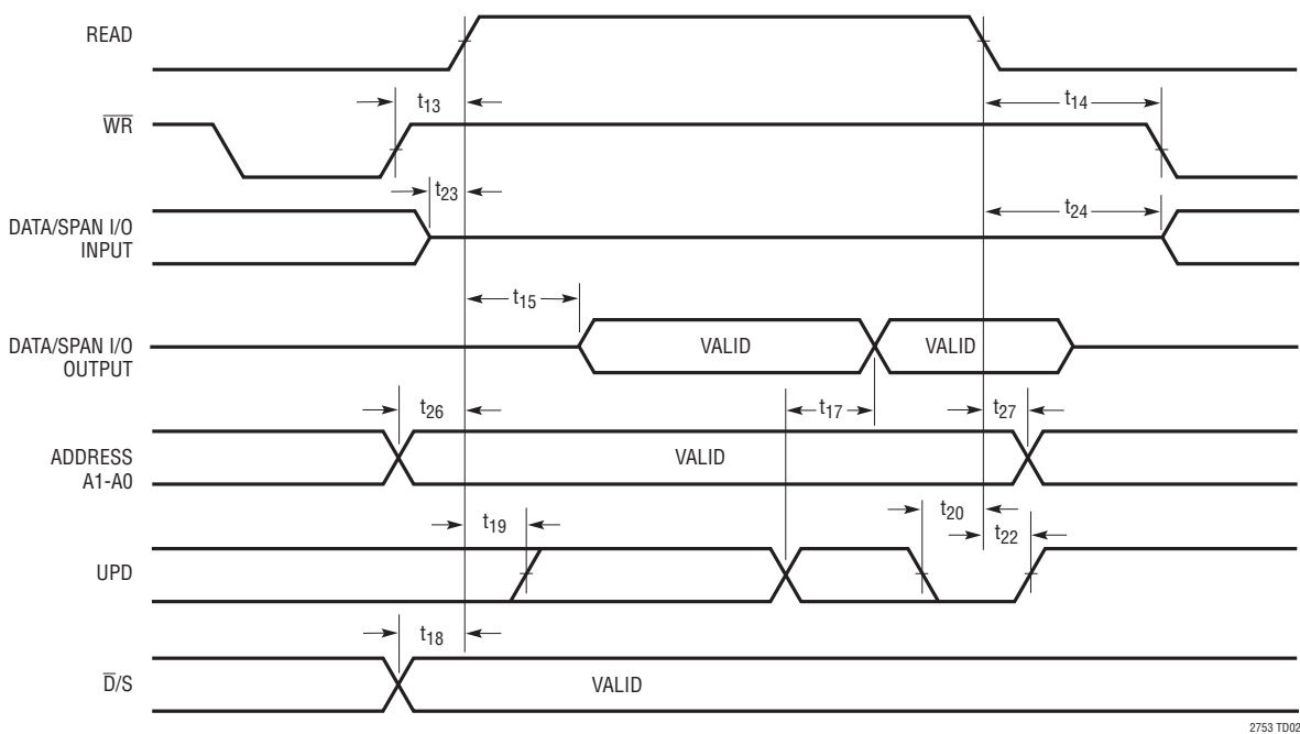
Readback Timing
